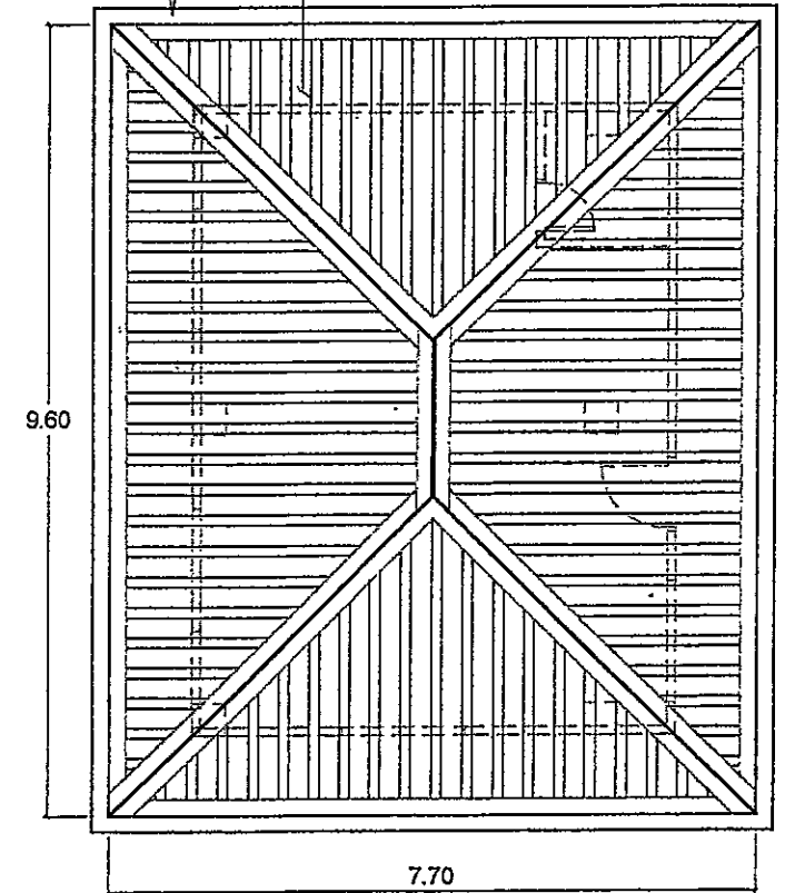
ROOF PLAN
